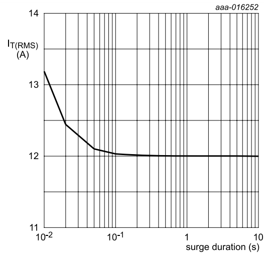
f = 50\text{ Hz} ; T_{mb} = 125\text{ °C} Fig. 2. RMS on-state current as a function of surge duration; maximum values
