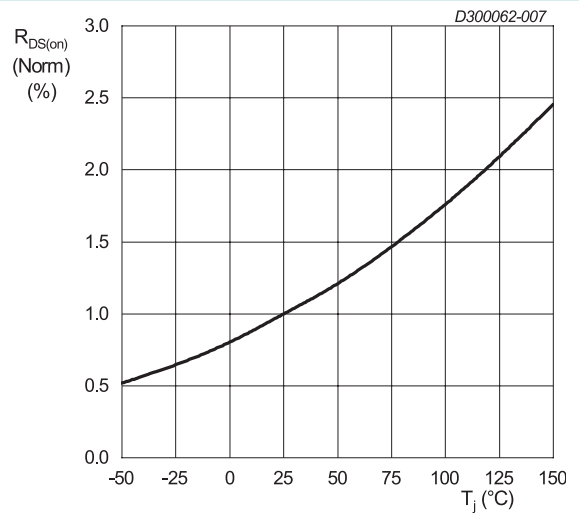
Fig. 7. Normalized drain-source on-state resistance as a function of junction temperature V_{GS} = 10\text{ V}; I_D = 15\text{ A}
